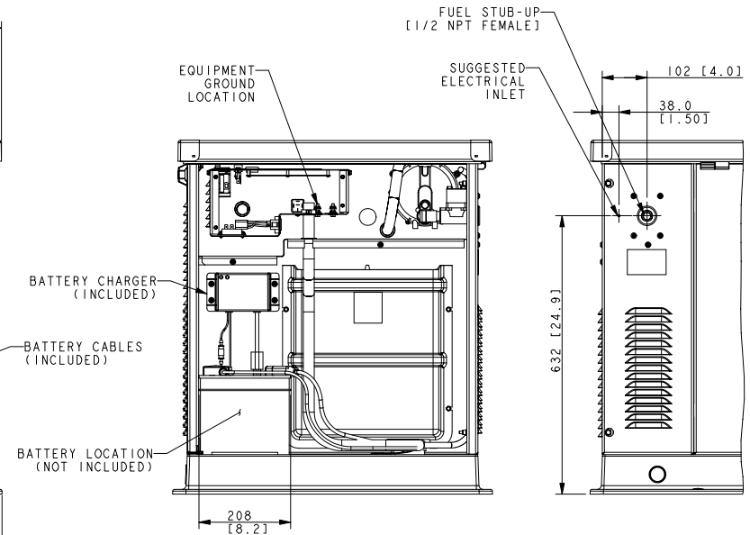
FRONT VIEW (END PANEL REMOVED TO SHOW DETAIL)
