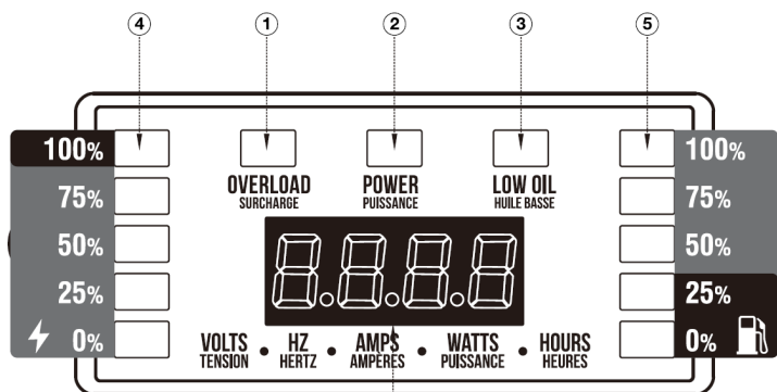
AUTOMATIC ROTATING DIGITAL DISPLAY(scroll once every 3 s)
